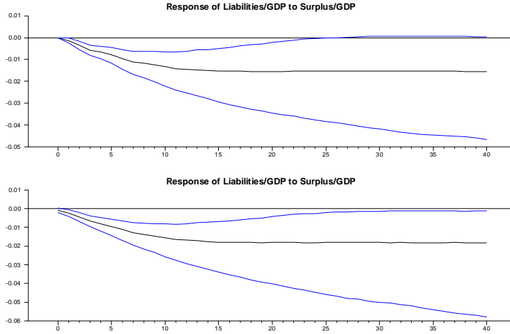
Figure 2: VAR impulse responses over the sample 1966Q1-2016Q1. Panel (a) ordering: Liabilities/GDP, Surplus/GDP. Panel (b) ordering: Surplus/GDP, Liabilities/GDP.
